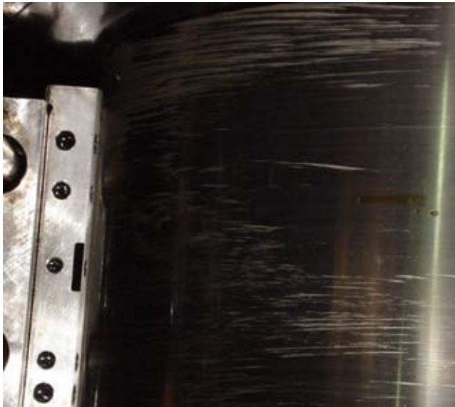
Main bearing journal
