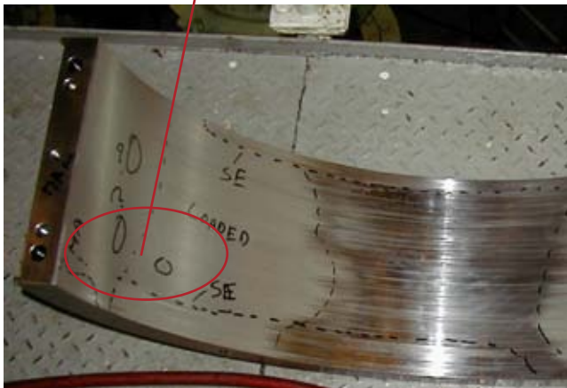
Corresponding lower bearing shell. Visible spark erosion, but no or limited wear can be measured.
