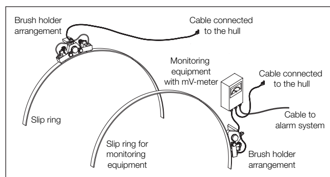
Shaftline earthing device parts
