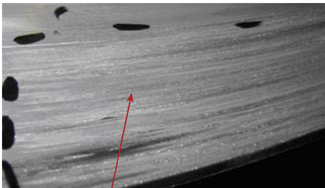
Main bearing journal
